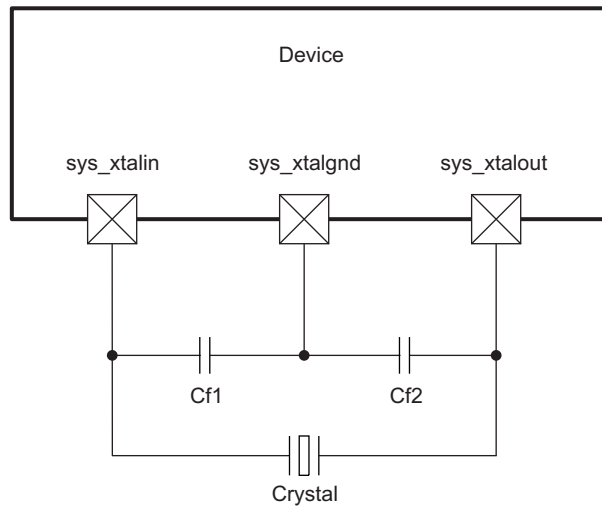
Figure 4-2. Crystal Implementation
