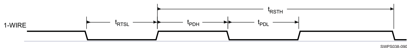
Figure 6-60. 1-Wire Reset Timing
