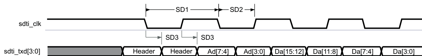
Figure 6-80. SDTI—Dual-Edge Mode
